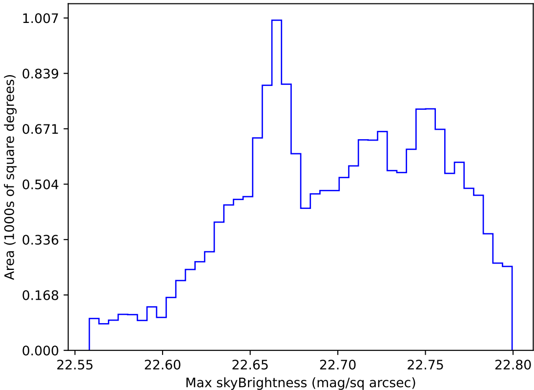
weather_cloudso0v3.5_10yrs WFD u band: Max skyBrightness
