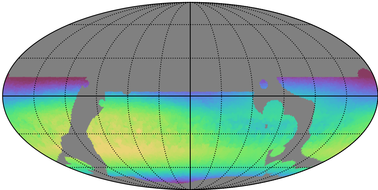
weather_cloudso0v3.5_10yrs WFD i band: Max skyBrightness
