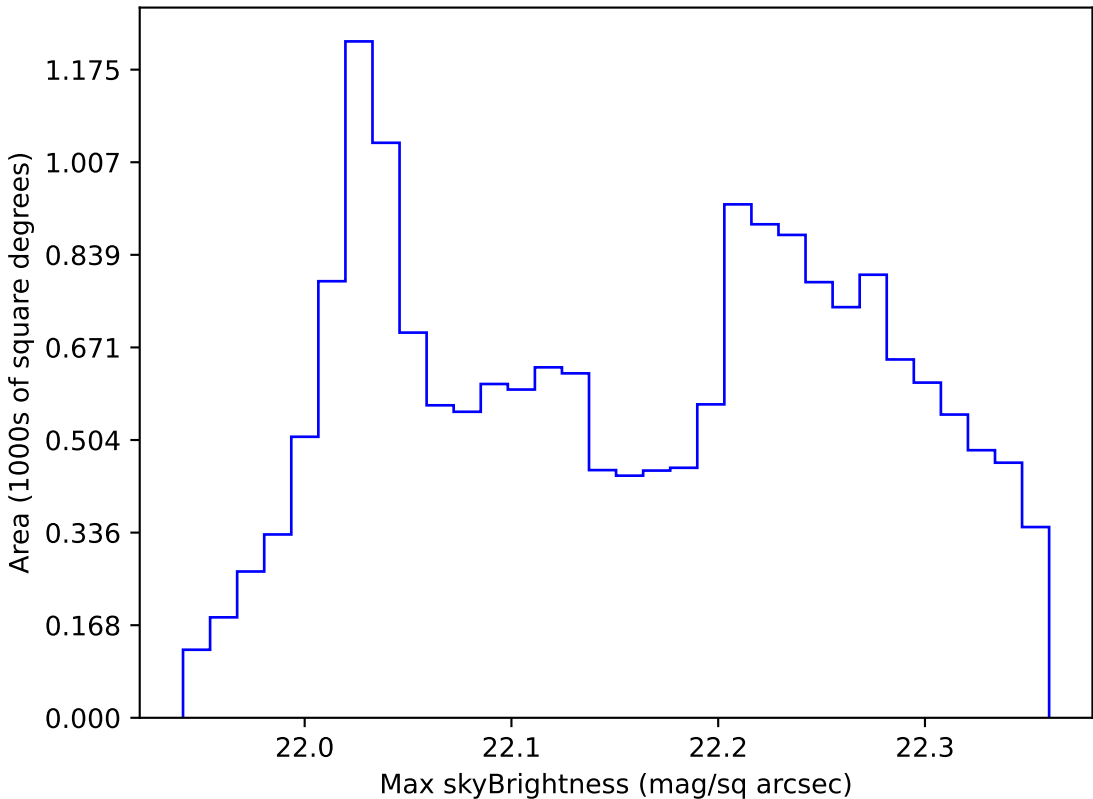
weather_cloudso0v3.5_10yrs WFD g band: Max skyBrightness
