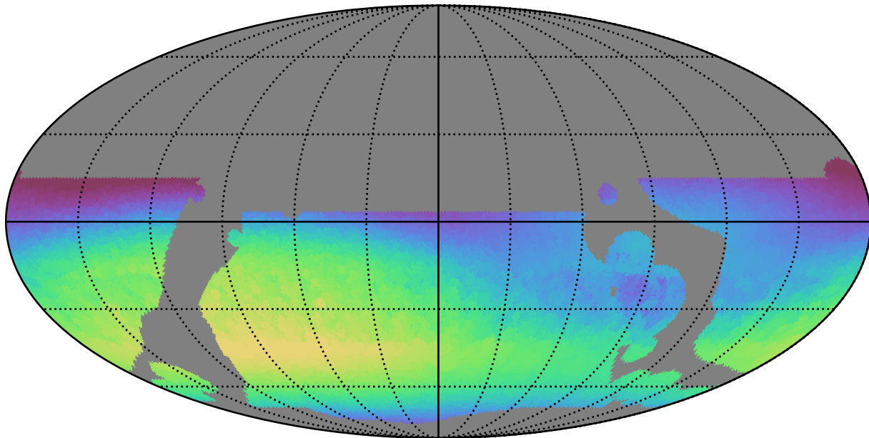
weather_cloudso0v3.5_10yrs WFD all bands: Max skyBrightness
