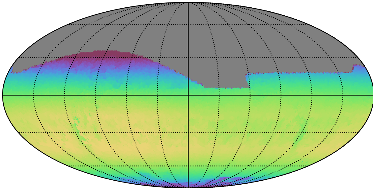
weather_cloudso0v3.5_10yrs All sky z band: Max skyBrightness
