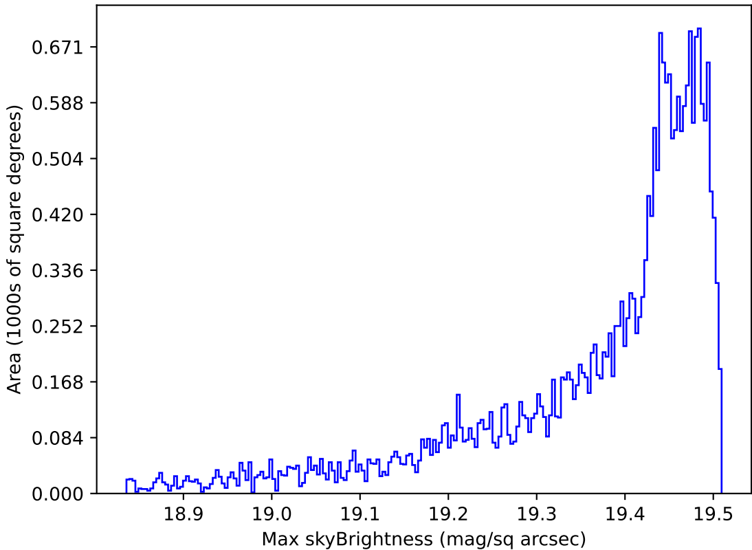
weather_cloudso0v3.5_10yrs All sky z band: Max skyBrightness
