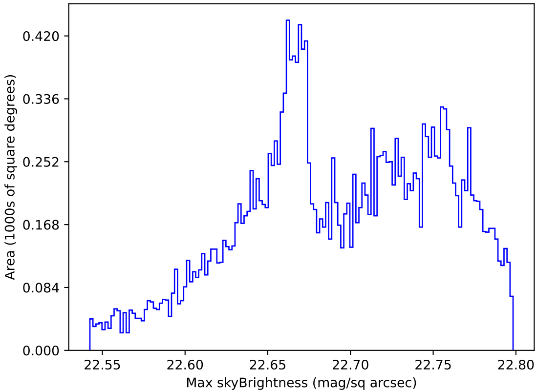
weather_cloudso0v3.5_10yrs All sky u band: Max skyBrightness
