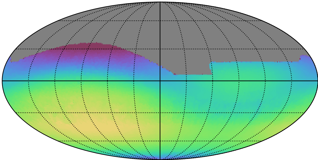
weather_cloudso0v3.5_10yrs All sky r band: Max skyBrightness
