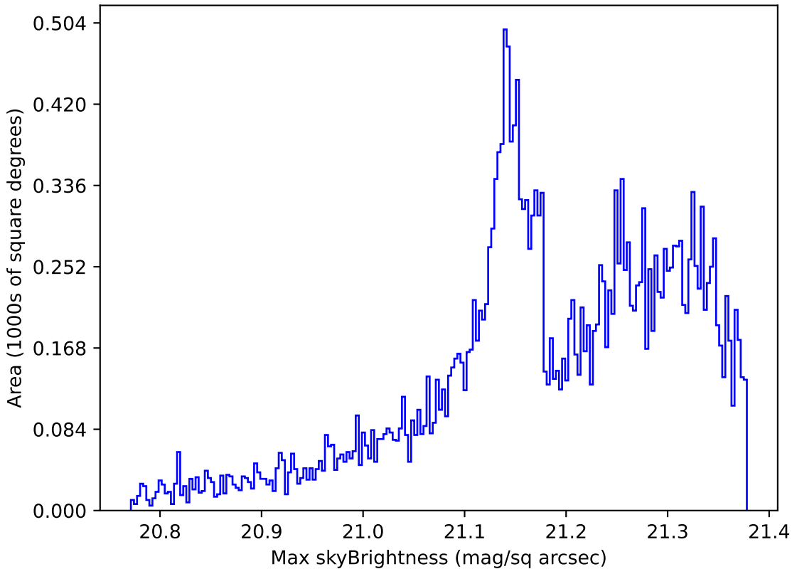
weather_cloudso0v3.5_10yrs All sky r band: Max skyBrightness
