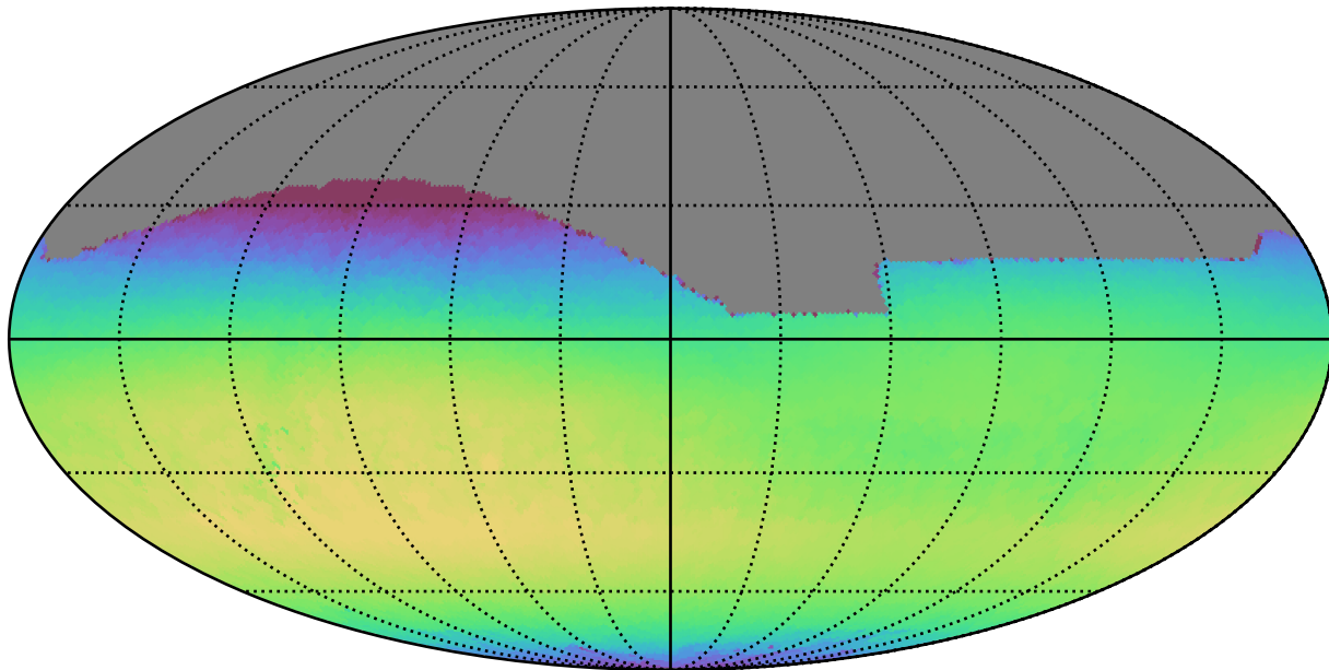
weather_cloudso0v3.5_10yrs All sky i band: Max skyBrightness
