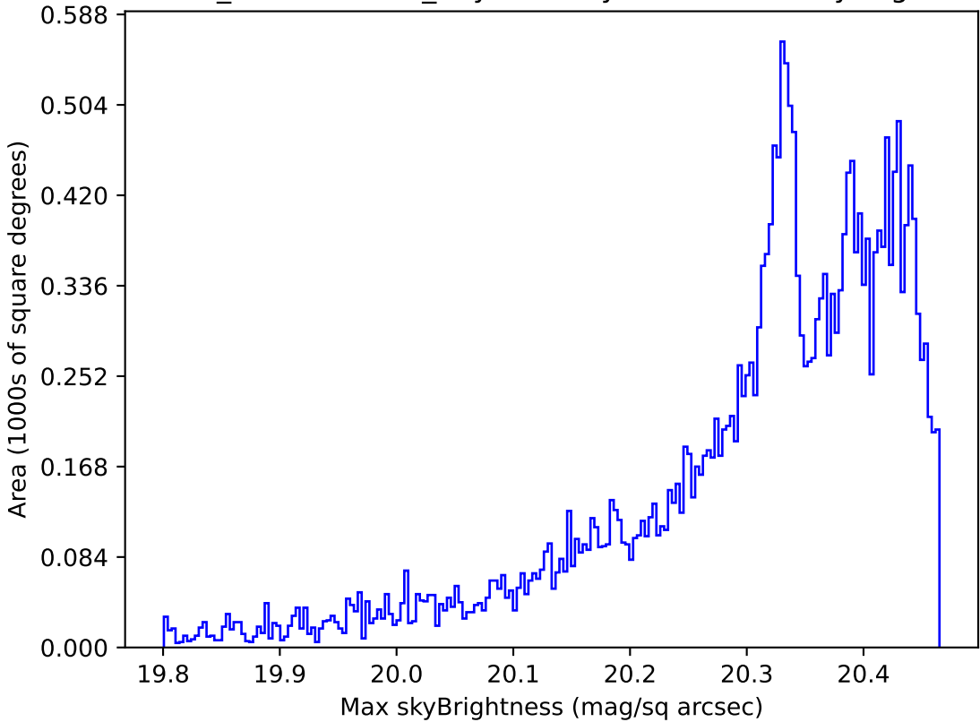
weather_cloudso0v3.5_10yrs All sky i band: Max skyBrightness
