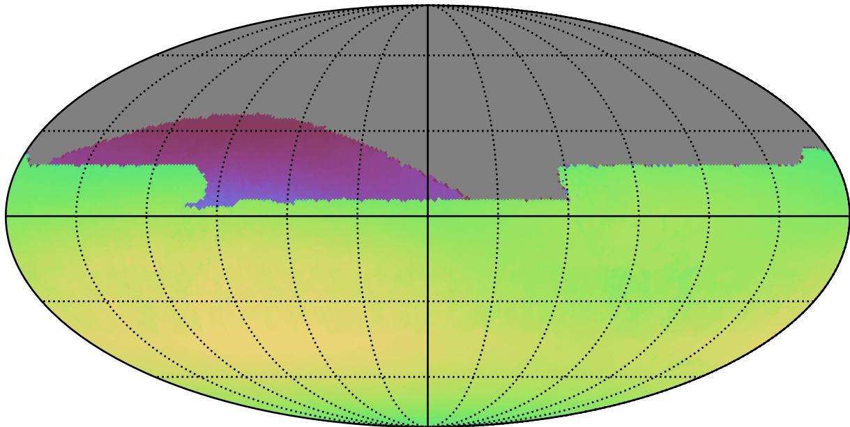
weather_cloudso0v3.5_10yrs All sky all bands: Max skyBrightness
