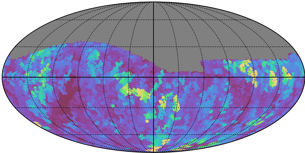
weather_cloudso0v3.5_10yrs Yr 1 z band: Max seeingGeom
