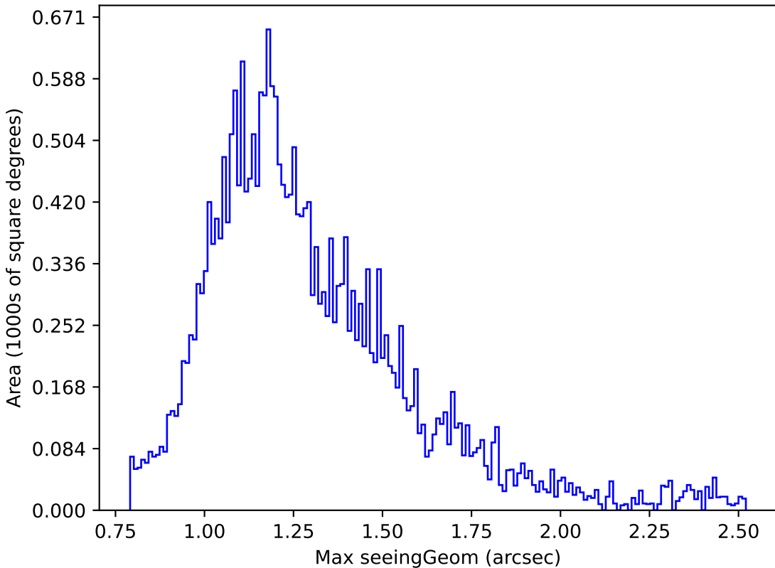
weather_cloudso0v3.5_10yrs Yr 1 z band: Max seeingGeom
