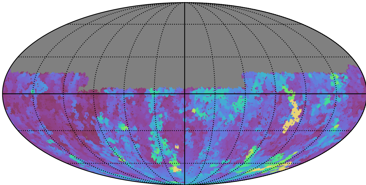
weather_cloudso0v3.5_10yrs Yr 1 u band: Max seeingGeom
