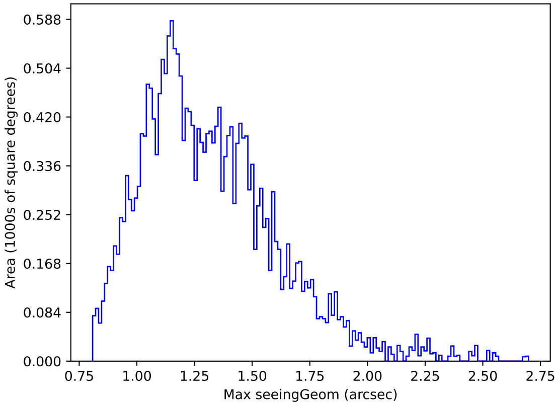
weather_cloudso0v3.5_10yrs Yr 1 u band: Max seeingGeom
