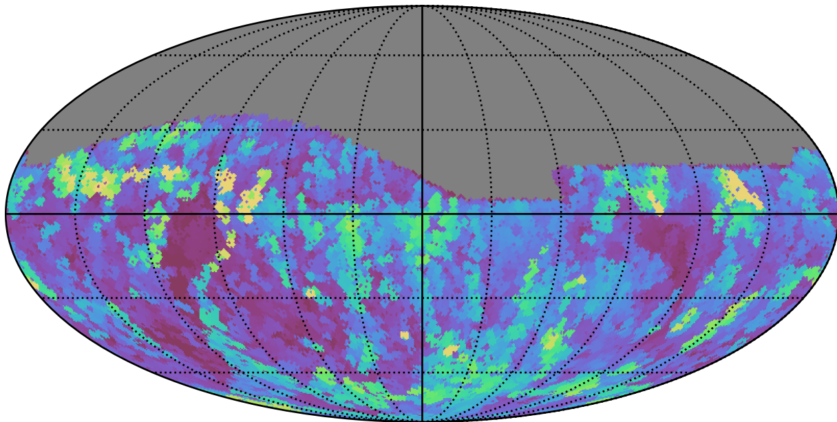
weather_cloudso0v3.5_10yrs Yr 1 r band: Max seeingGeom
