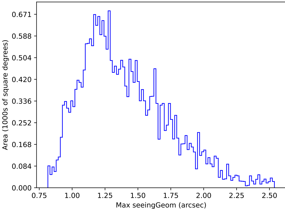
weather_cloudso0v3.5_10yrs Yr 1 r band: Max seeingGeom
