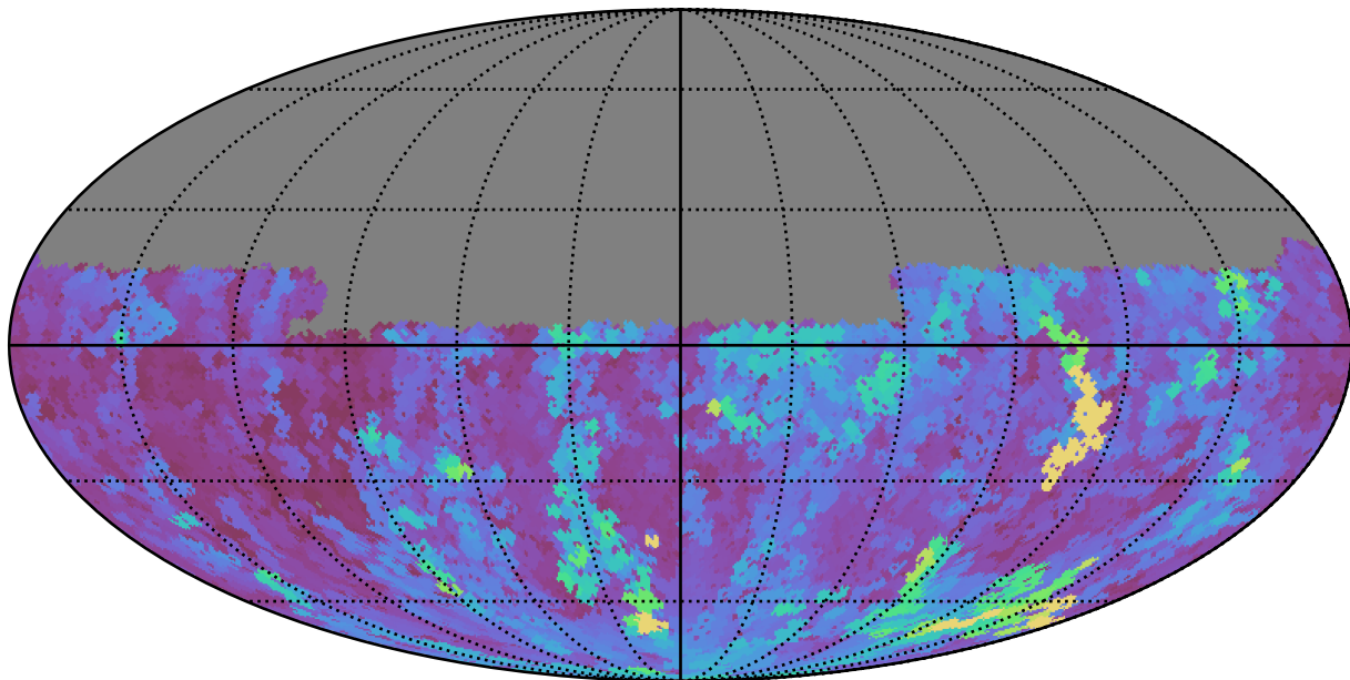
weather_cloudso0v3.5_10yrs Yr 1 u band: Max seeingEff
