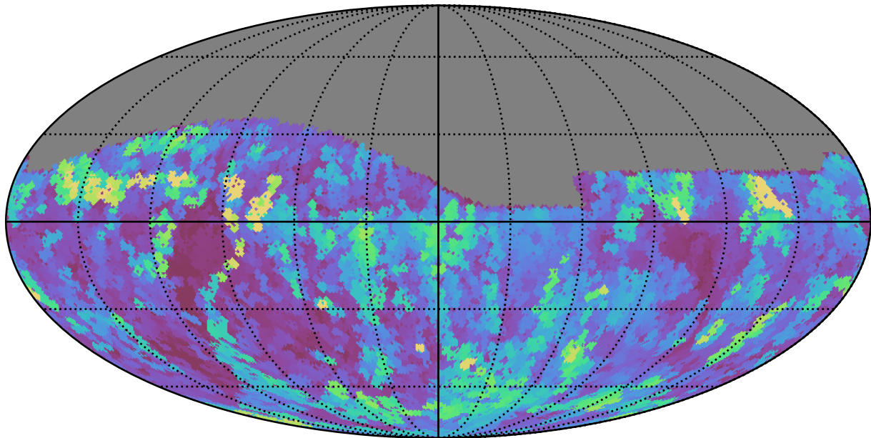
weather_cloudso0v3.5_10yrs Yr 1 r band: Max seeingEff
