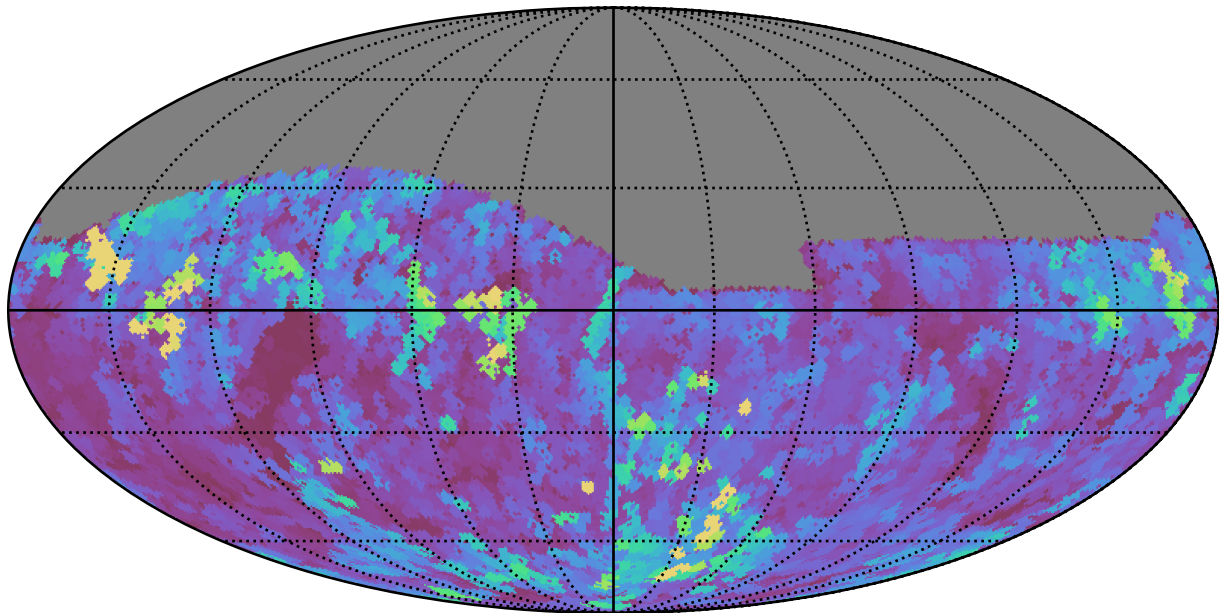
weather_cloudso0v3.5_10yrs Yr 1 i band: Max seeingEff
