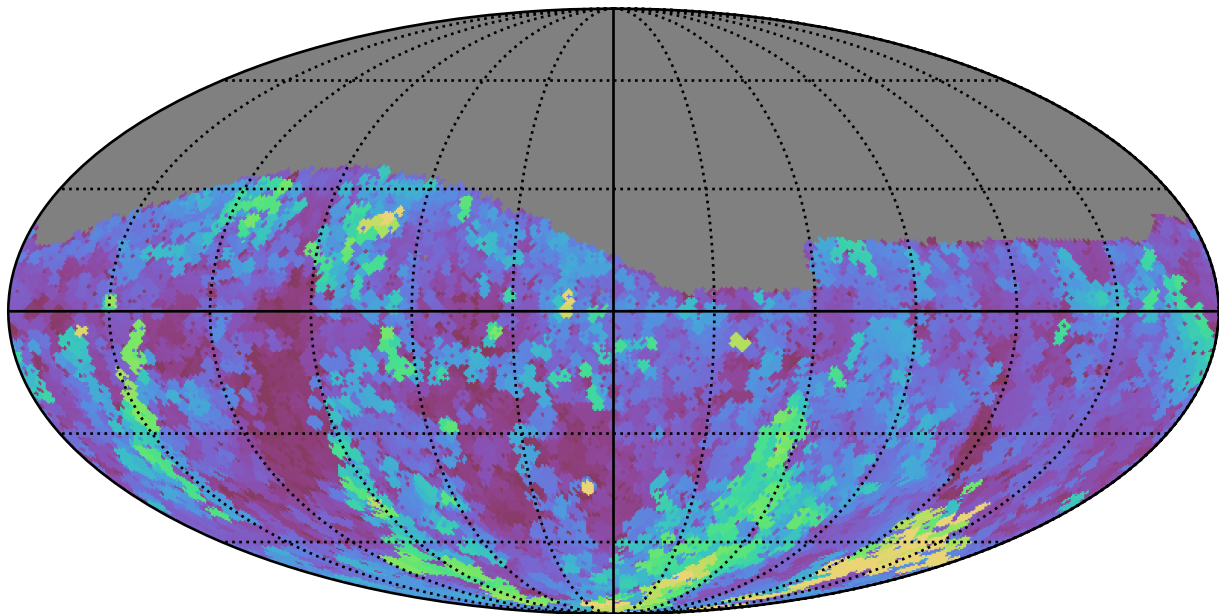
weather_cloudso0v3.5_10yrs Yr 1 g band: Max seeingEff
