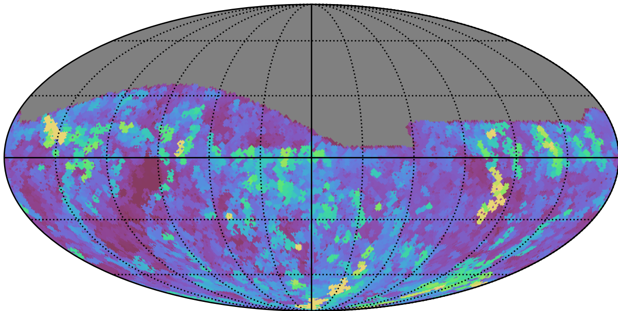
weather_cloudso0v3.5_10yrs Yr 1 all bands: Max seeingEff
