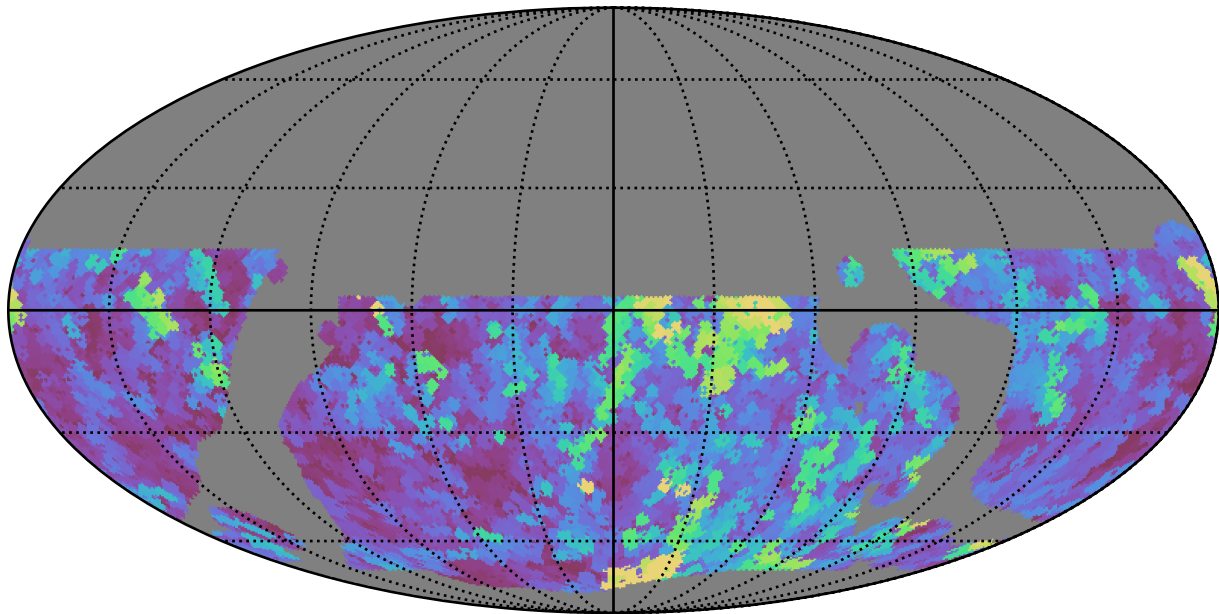
weather_cloudso0v3.5_10yrs WFD z band: Max seeingEff
