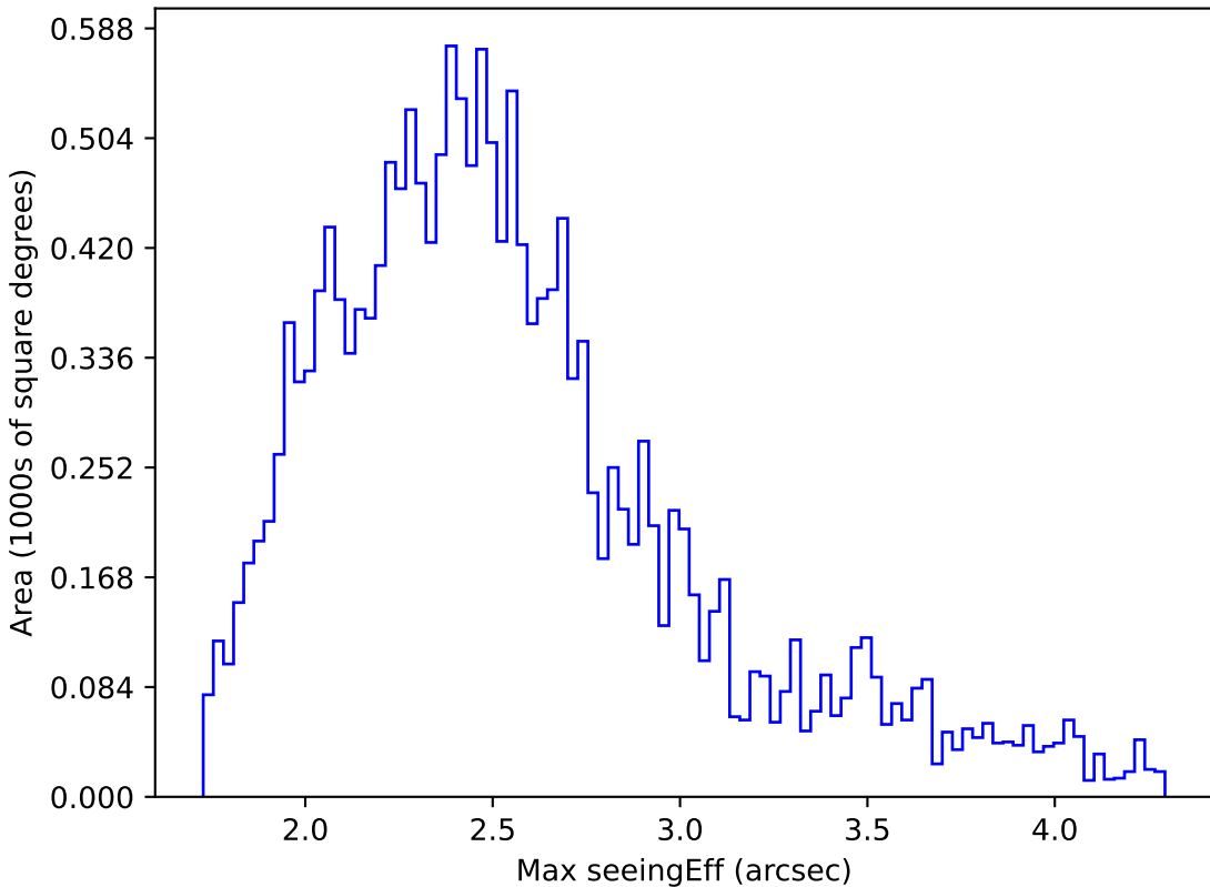
weather_cloudso0v3.5_10yrs WFD z band: Max seeingEff
