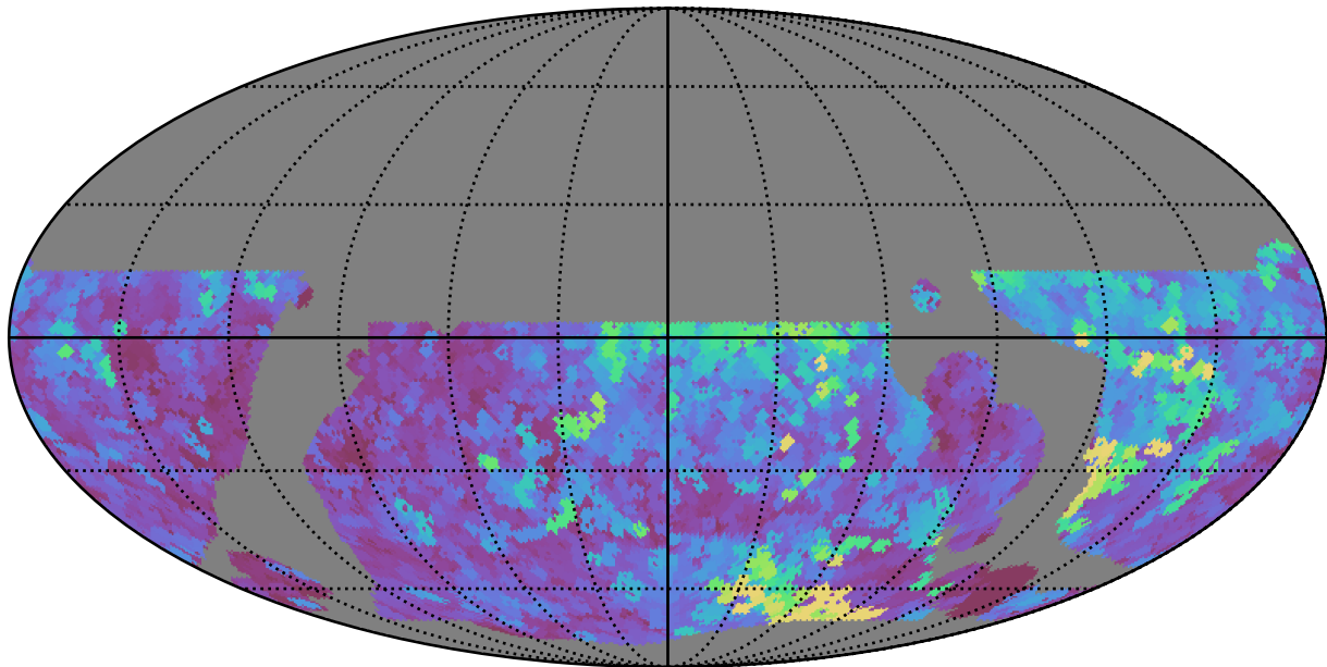
weather_cloudso0v3.5_10yrs WFD y band: Max seeingEff
