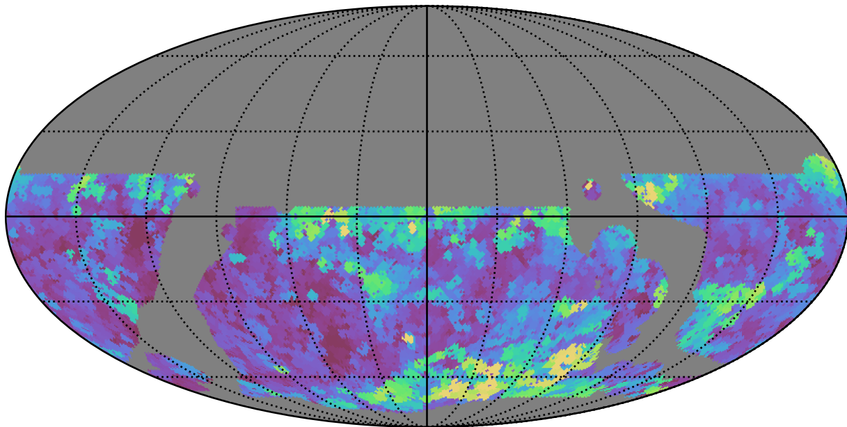
weather_cloudso0v3.5_10yrs WFD u band: Max seeingEff
