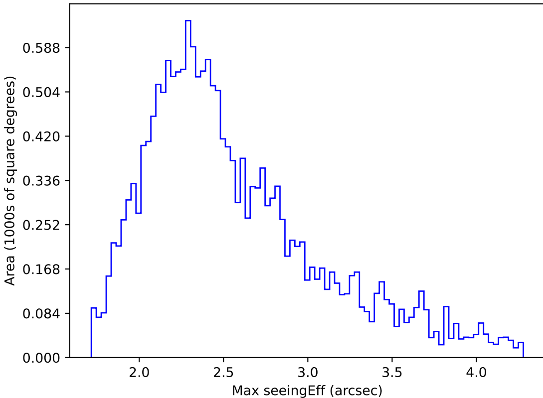
weather_cloudso0v3.5_10yrs WFD u band: Max seeingEff
