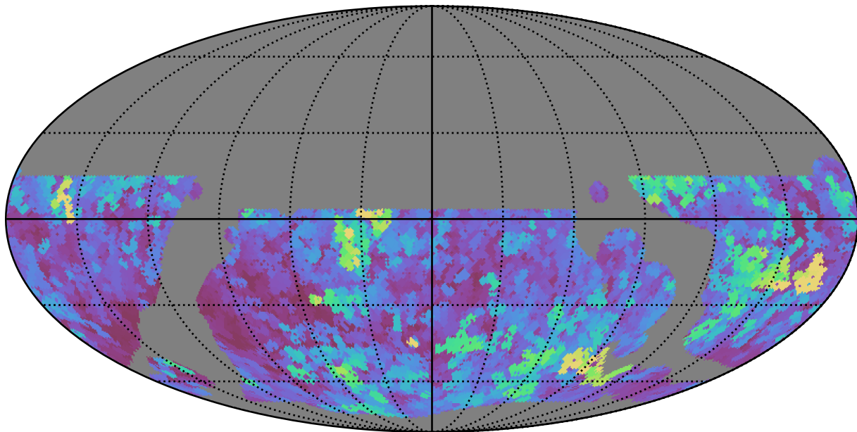
weather_cloudso0v3.5_10yrs WFD r band: Max seeingEff
