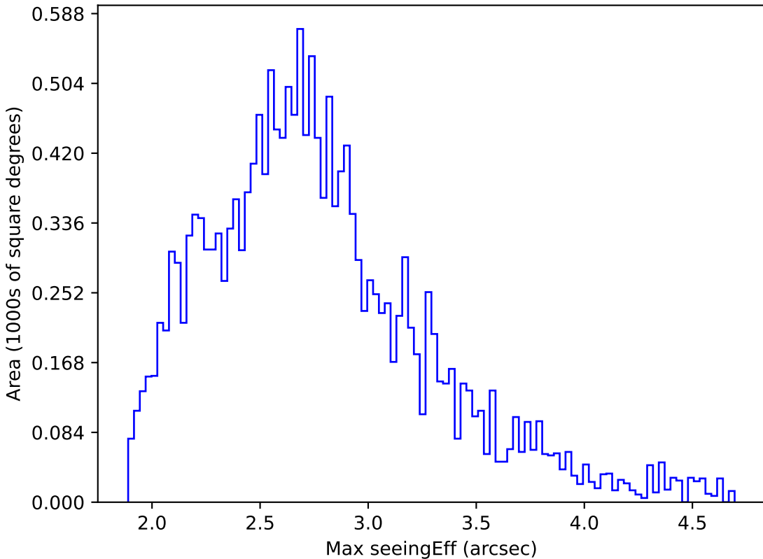
weather_cloudso0v3.5_10yrs WFD r band: Max seeingEff
