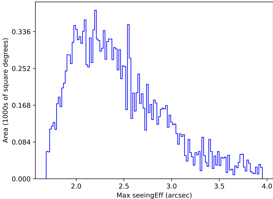
weather_cloudso0v3.5_10yrs WFD g band: Max seeingEff
