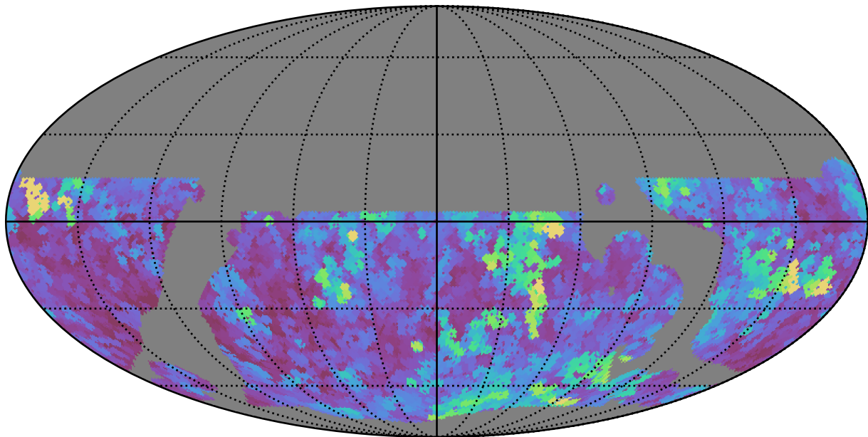
weather_cloudso0v3.5_10yrs WFD all bands: Max seeingEff
