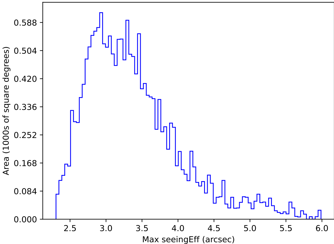
weather_cloudso0v3.5_10yrs WFD all bands: Max seeingEff
