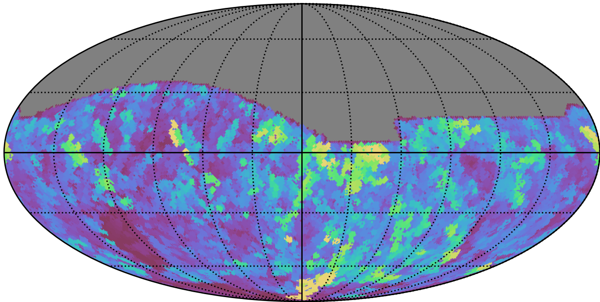
weather_cloudso0v3.5_10yrs All sky z band: Max seeingEff
