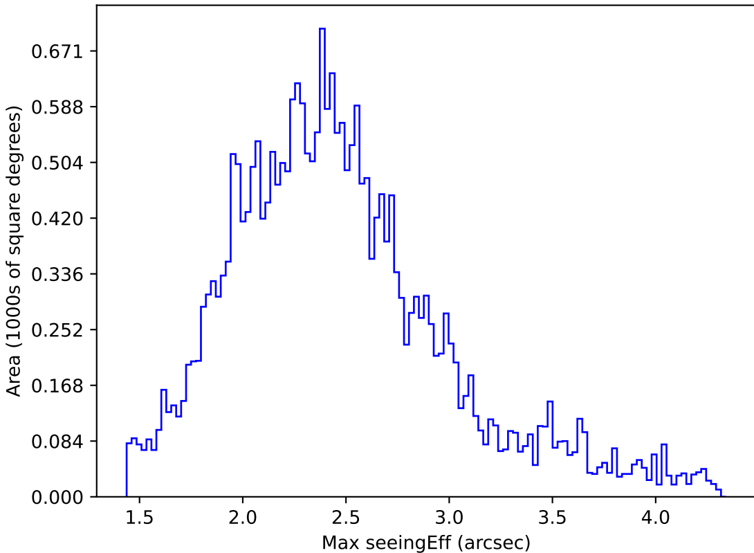
weather_cloudso0v3.5_10yrs All sky z band: Max seeingEff
