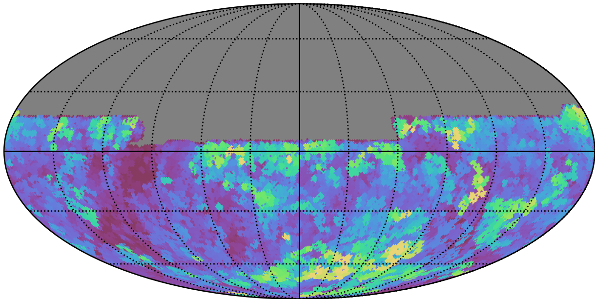
weather_cloudso0v3.5_10yrs All sky u band: Max seeingEff
