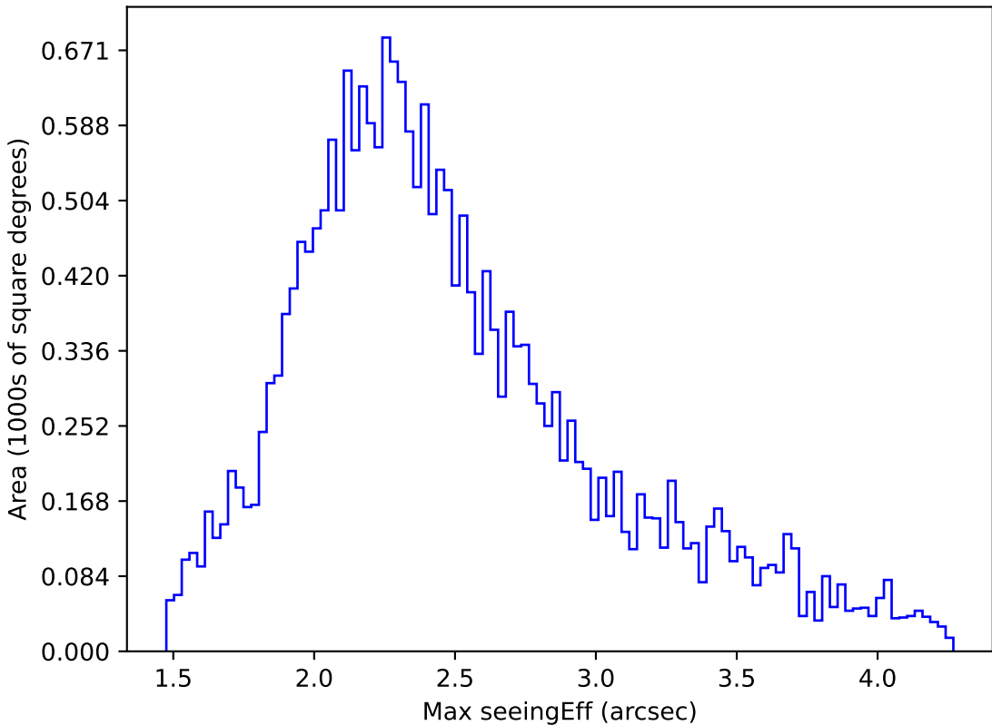
weather_cloudso0v3.5_10yrs All sky u band: Max seeingEff
