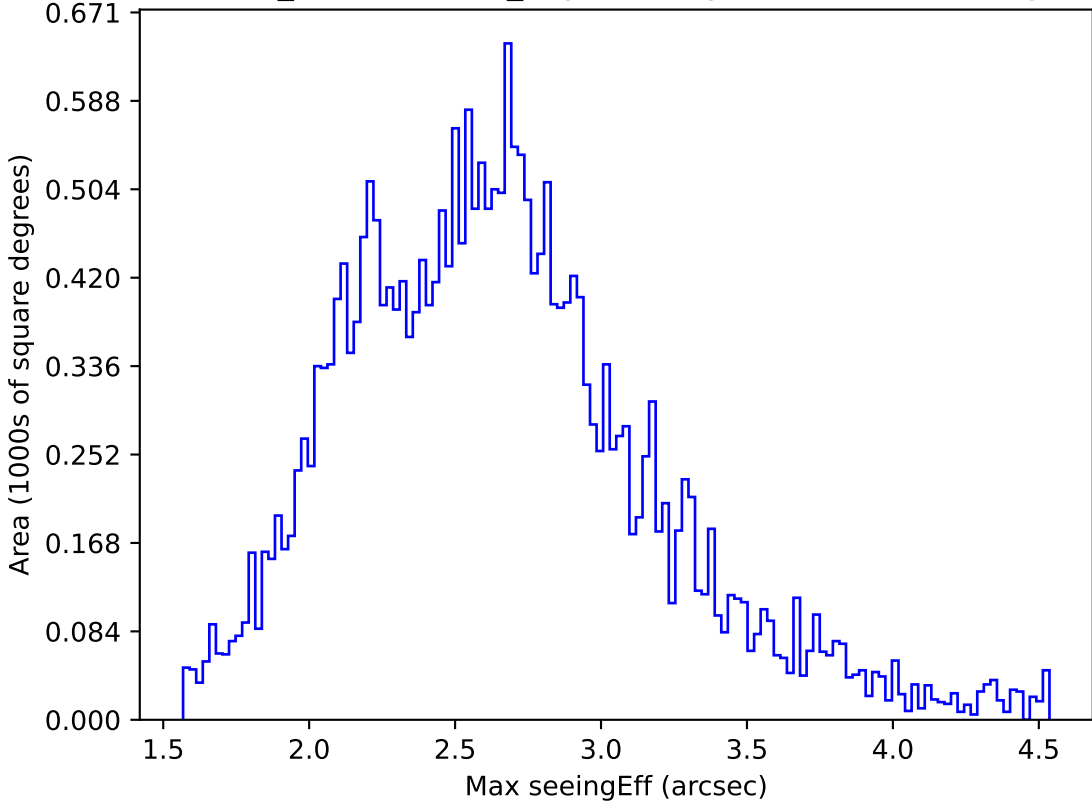
weather_cloudso0v3.5_10yrs All sky r band: Max seeingEff
