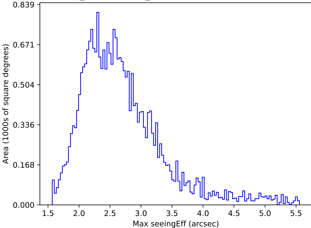
weather_cloudso0v3.5_10yrs All sky i band: Max seeingEff
