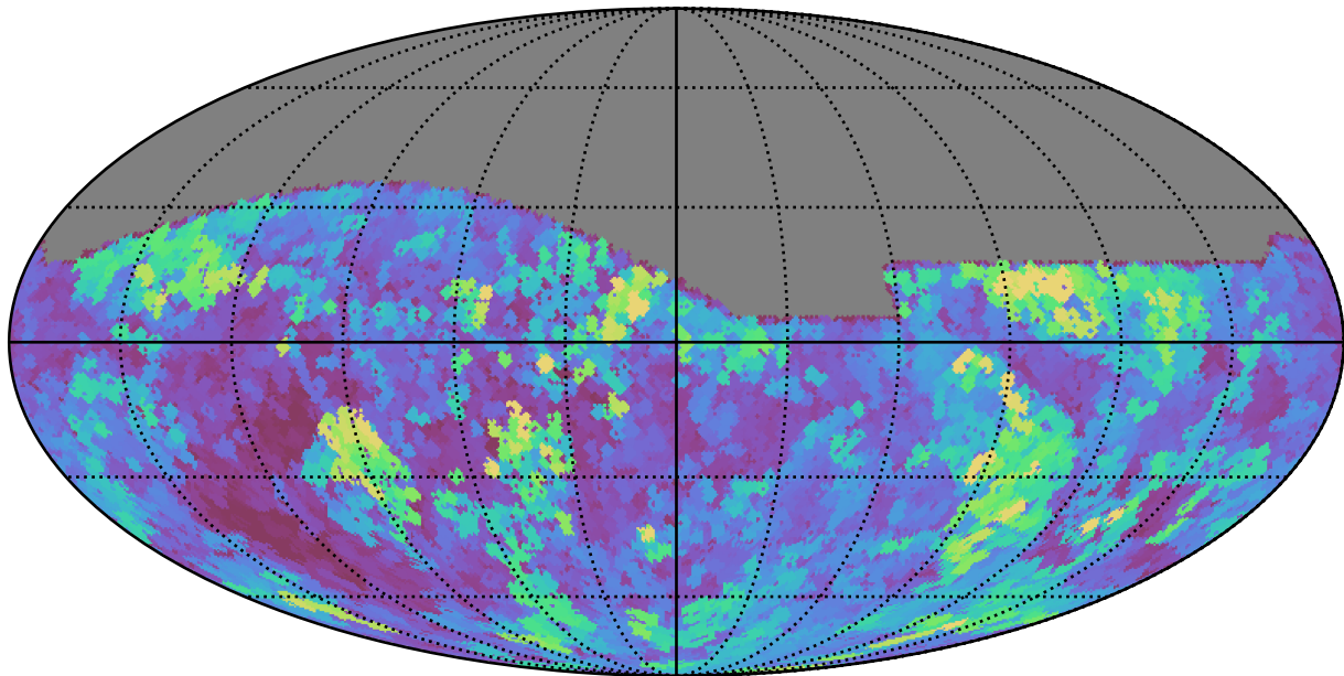
weather_cloudso0v3.5_10yrs All sky g band: Max seeingEff
