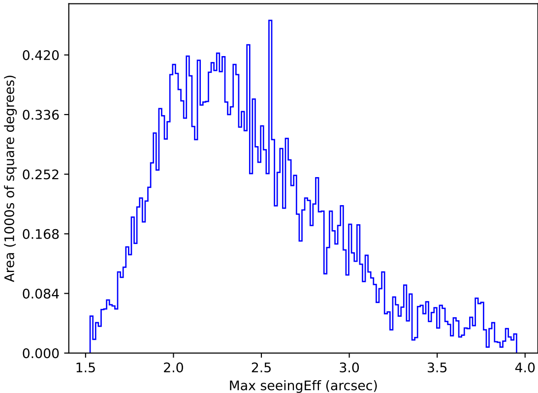
weather_cloudso0v3.5_10yrs All sky g band: Max seeingEff
