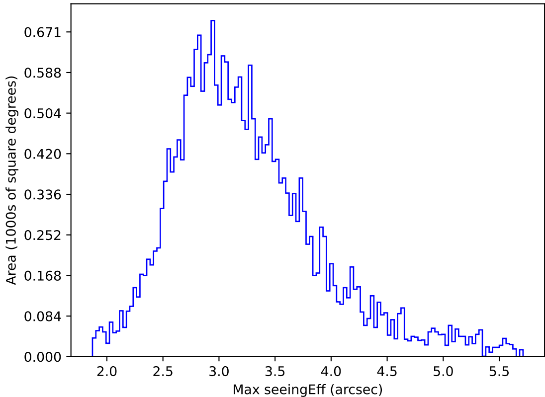
weather_cloudso0v3.5_10yrs All sky all bands: Max seeingEff
