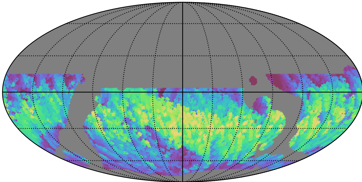
weather_cloudso0v3.5_10yrs WFD z band: Max normairmass
