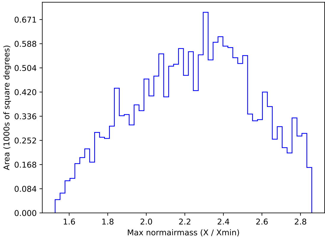
weather_cloudso0v3.5_10yrs WFD z band: Max normairmass
