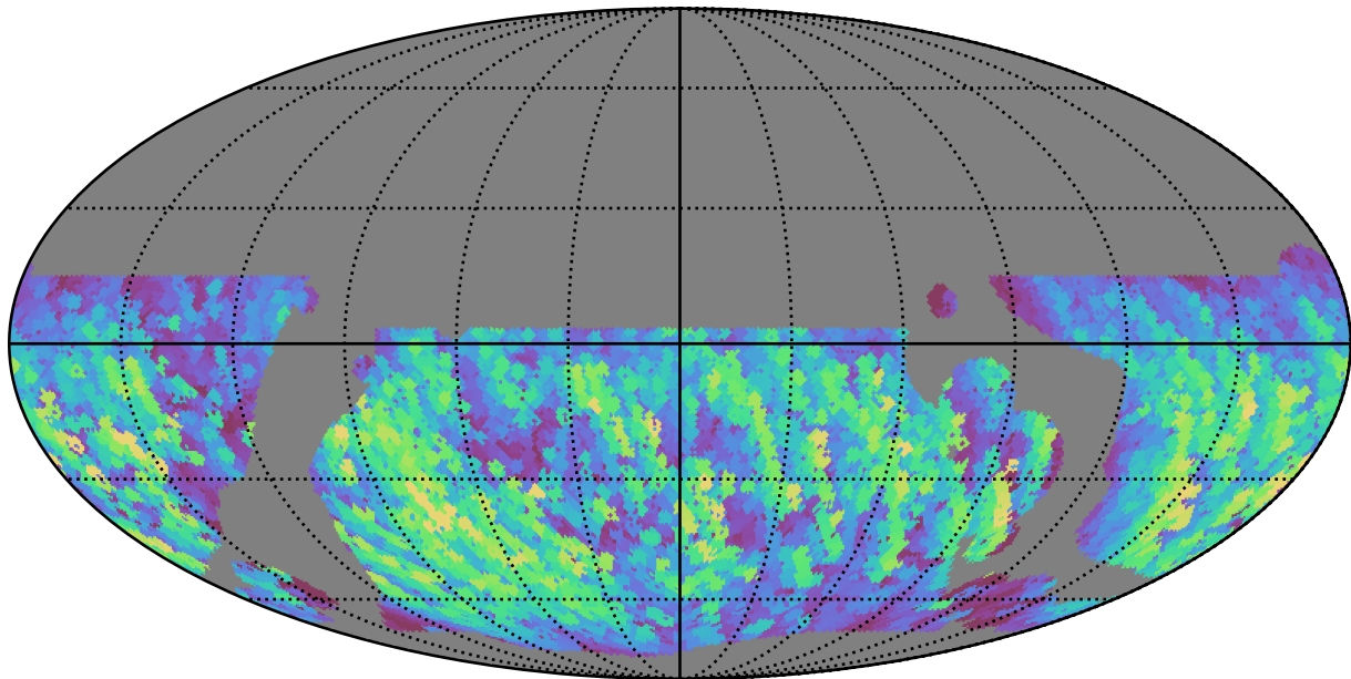
weather_cloudso0v3.5_10yrs WFD y band: Max normairmass
