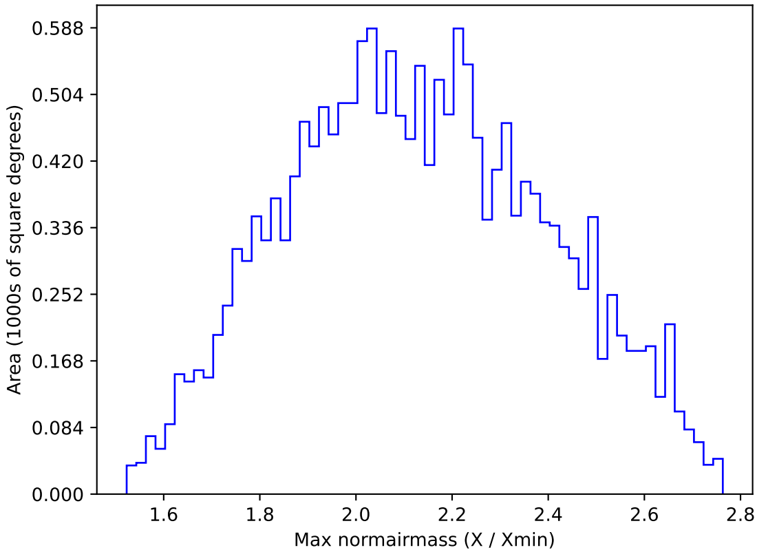
weather_cloudso0v3.5_10yrs WFD y band: Max normairmass
