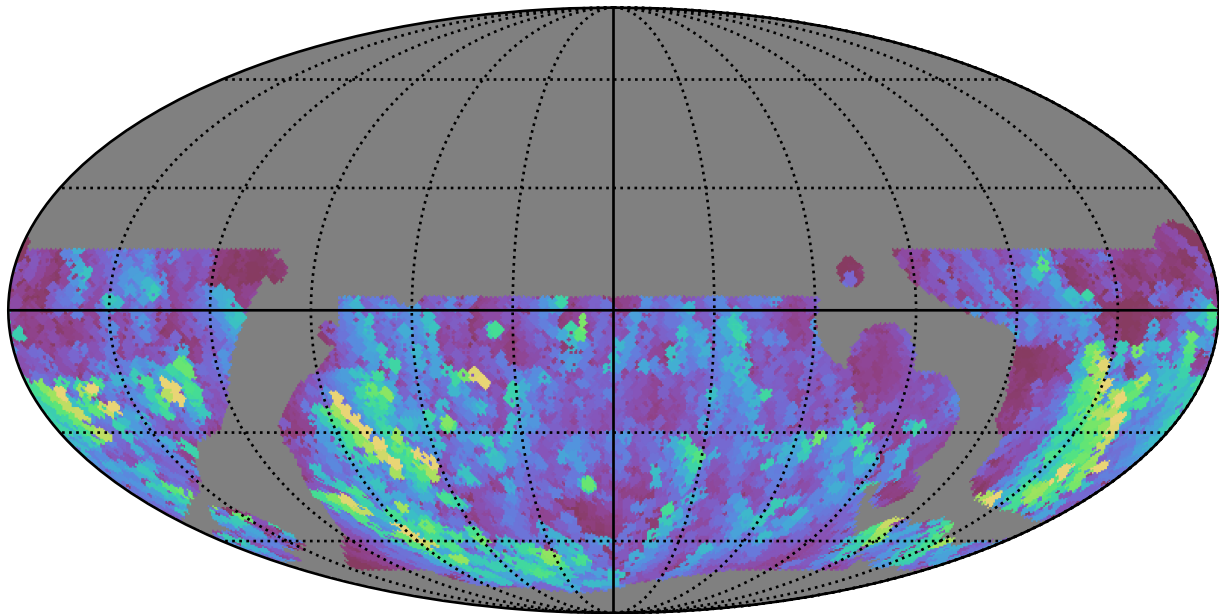
weather_cloudso0v3.5_10yrs WFD u band: Max normairmass
