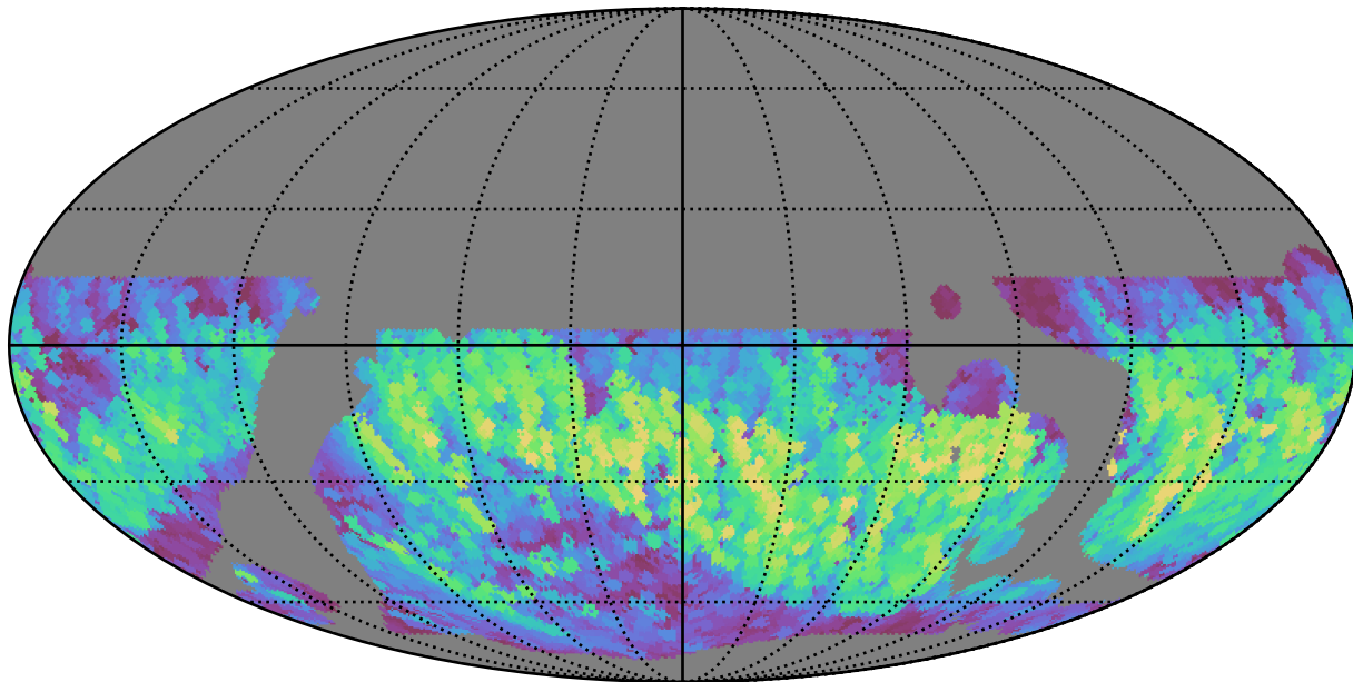
weather_cloudso0v3.5_10yrs WFD r band: Max normairmass
