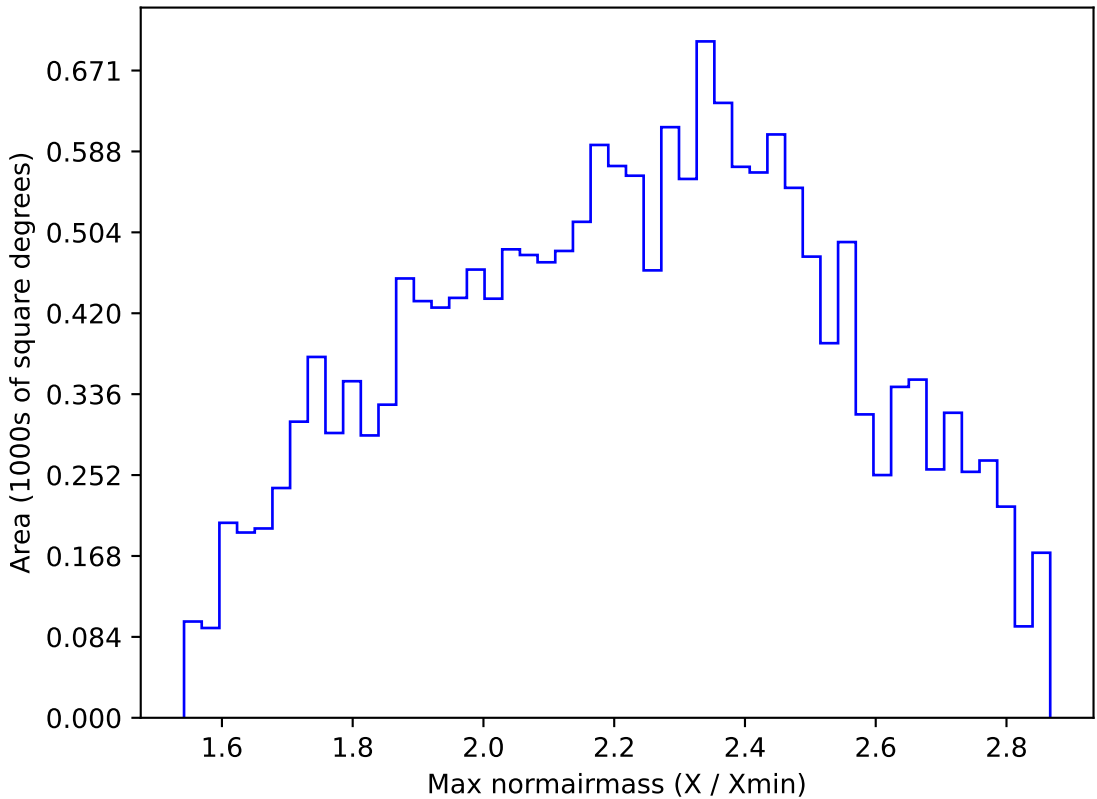
weather_cloudso0v3.5_10yrs WFD r band: Max normairmass
