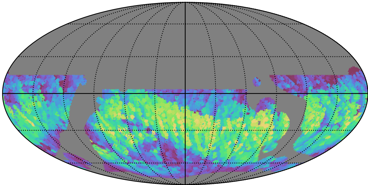
weather_cloudso0v3.5_10yrs WFD i band: Max normairmass
